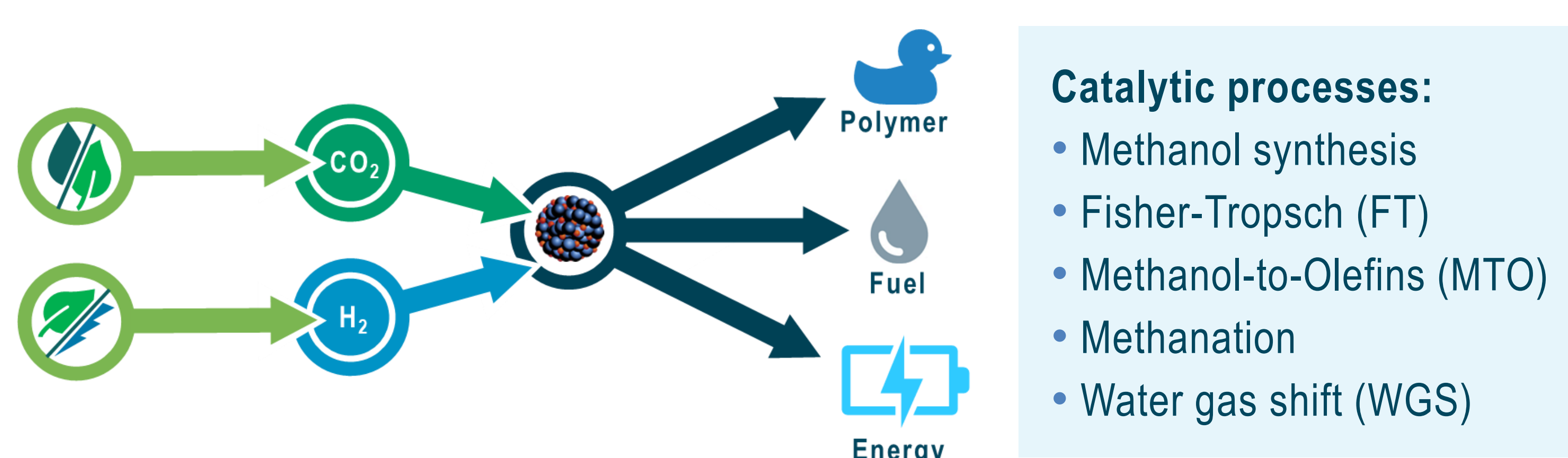
Figure 4. Utilization of renewable CO 2 and H 2 using different catalytic processes offered by hte
