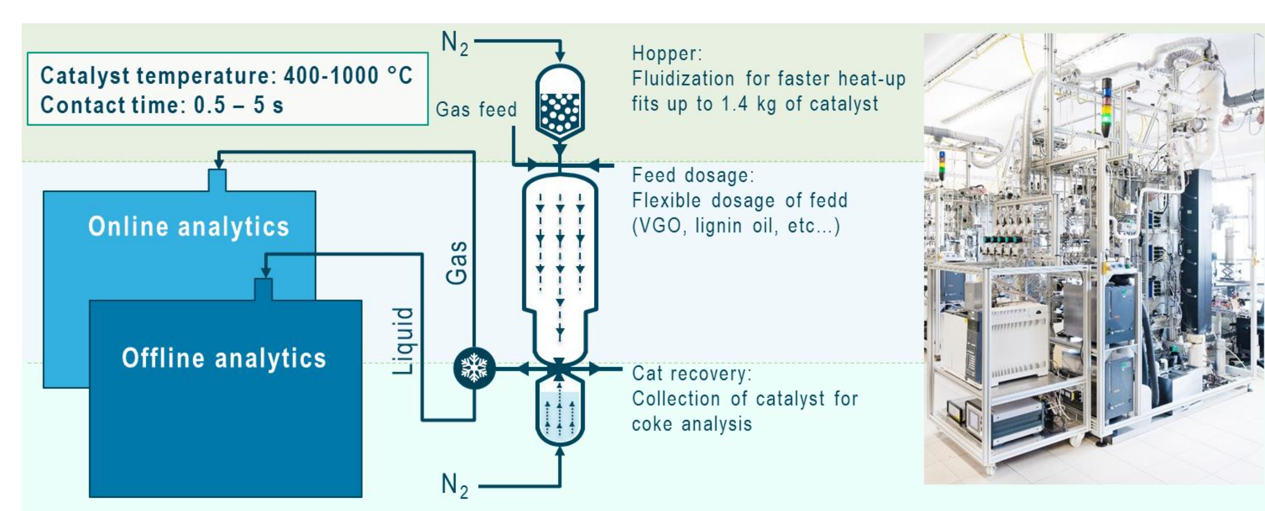
Figure 2. Micro down flow unit at hte. Thermal and catalytic cracking of different feeds can be carried on in a similar way to the FCC unit
